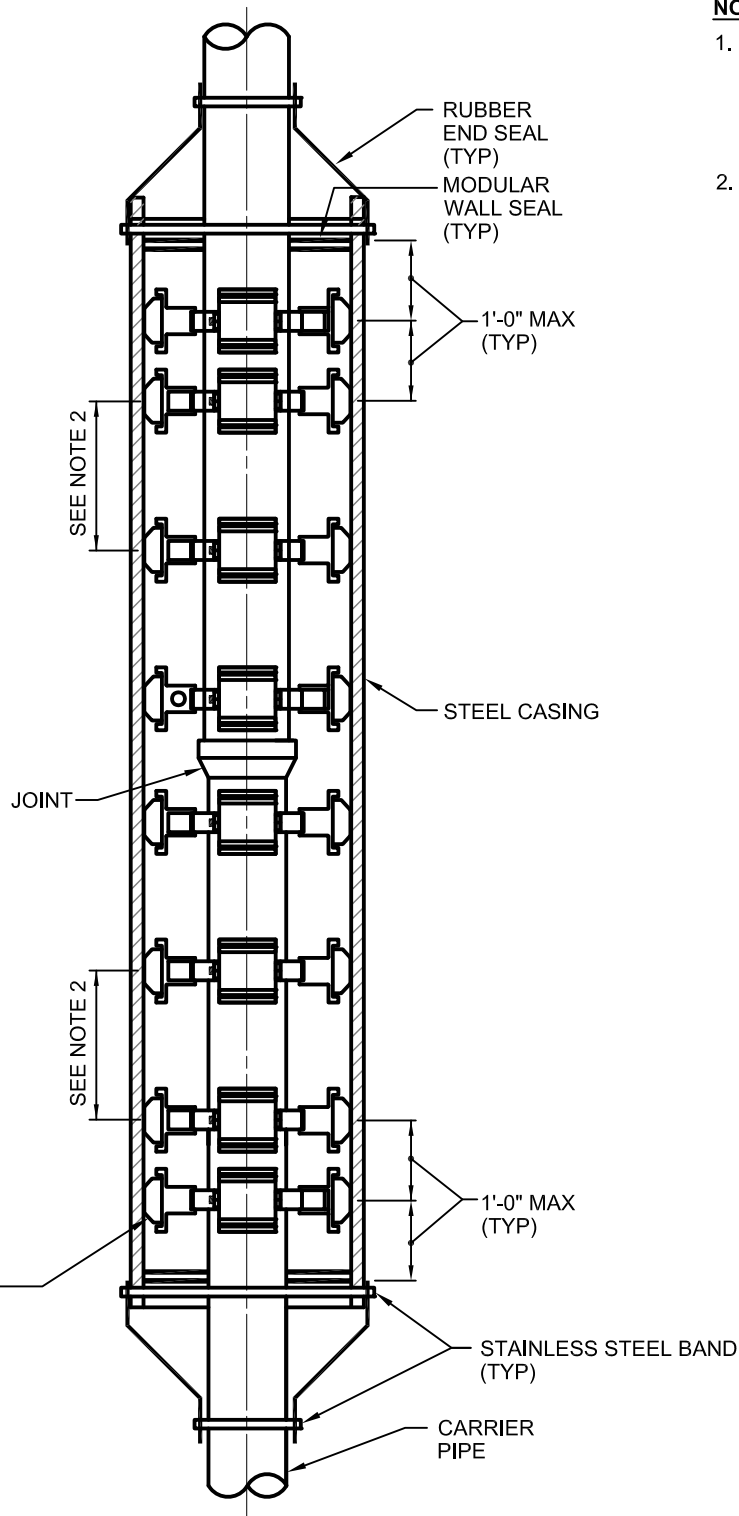
PIPE CASING DETAIL NOT TO SCALE
